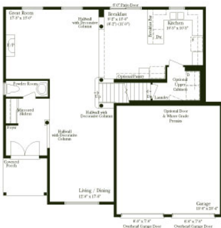
GROUND FLOOR PLAN ELEVATION 'A'
